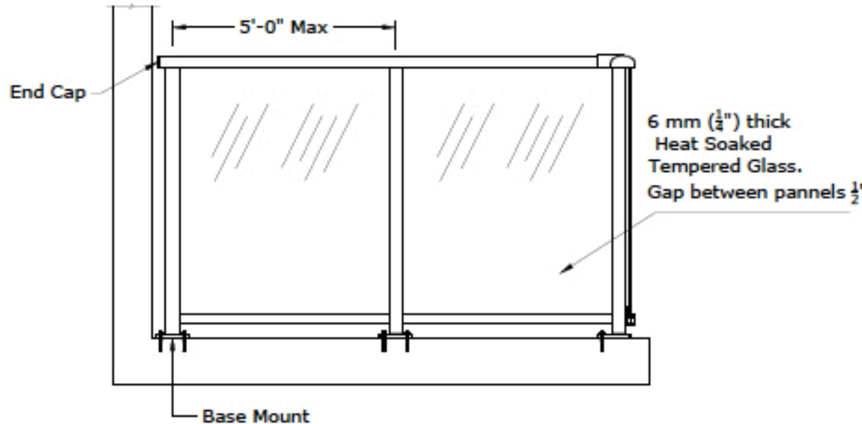
Balcony / Porch Railing Section
