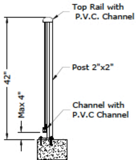
Balcony / Porch Railing Section
